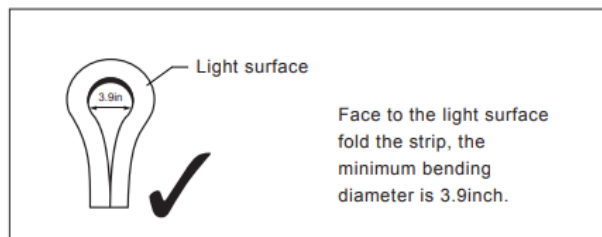
Correct Bending Way
